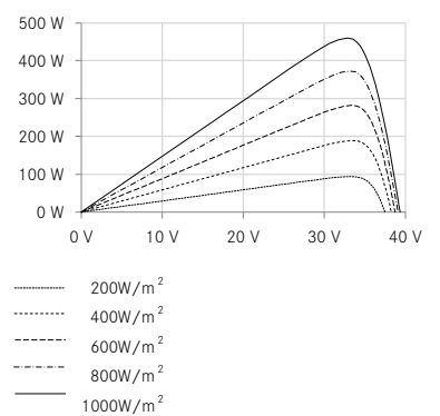
UP-Kennlinie Bsp. 460 Wp
